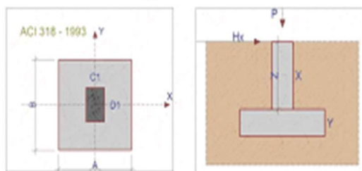
SINGLE FOOTING (PROKON)
